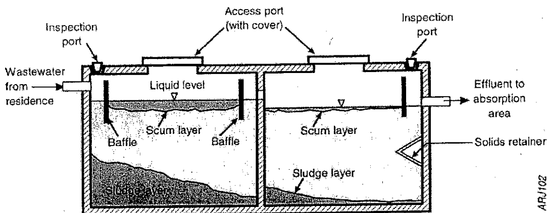
Figure 1. Cross-section of a two-chamber septic tank.
